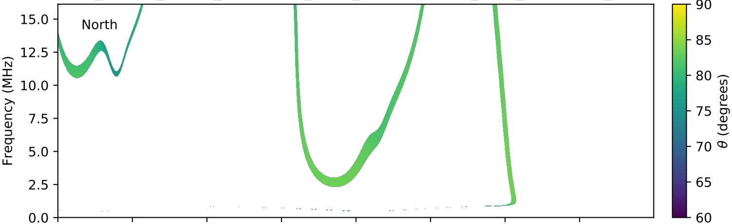
expres_cassini_jupiter_ganymede_isaac_lossc-wid1deg_3kev_20030829_v01.cdf
