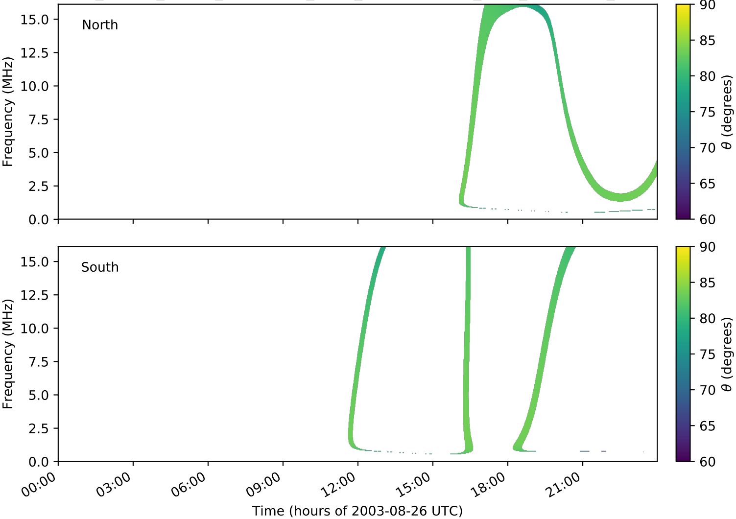
expres_cassini_jupiter_ganymede_isaac_lossc-wid1deg_3kev_20030826_v01.cdf
