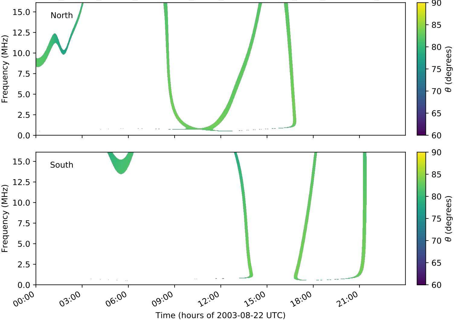
expres_cassini_jupiter_ganymede_isaac_lossc-wid1deg_3kev_20030822_v01.cdf
