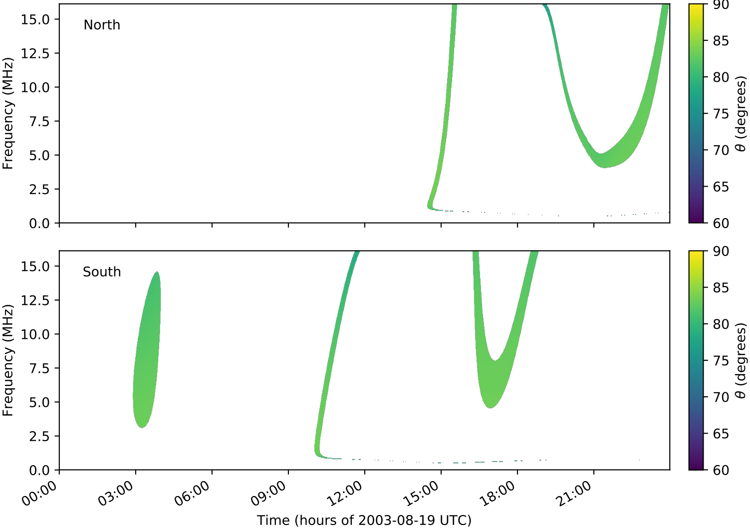
expres_cassini_jupiter_ganymede_isaac_lossc-wid1deg_3kev_20030819_v01.cdf
