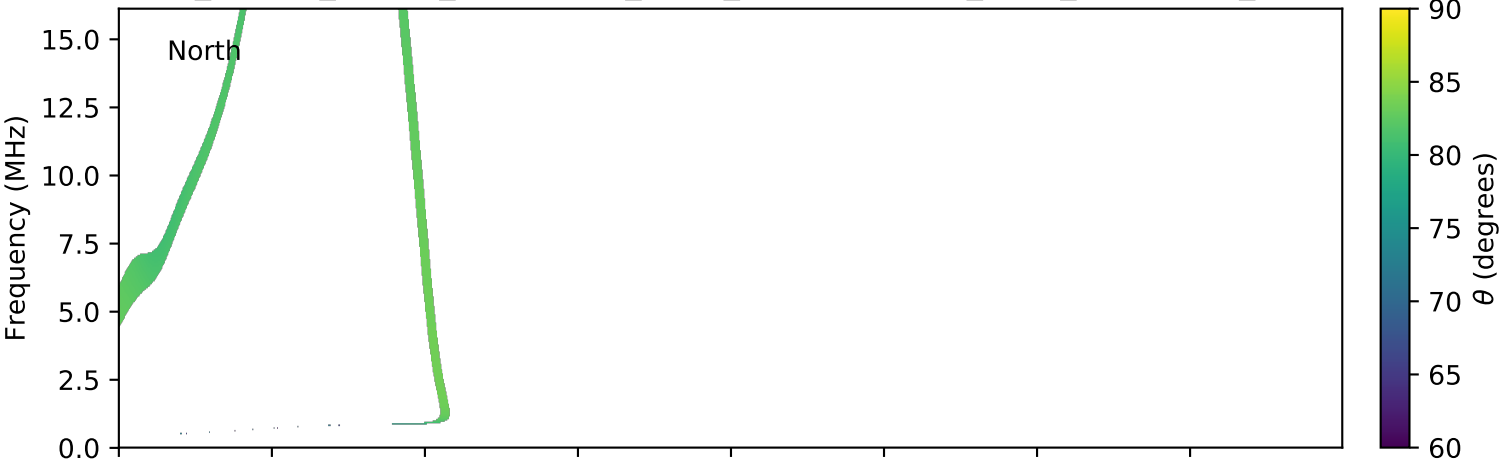
expres_cassini_jupiter_ganymede_isaac_lossc-wid1deg_3kev_20030808_v01.cdf
