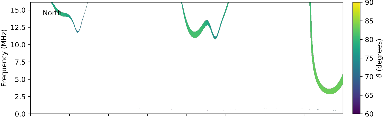
expres_cassini_jupiter_ganymede_isaac_lossc-wid1deg_3kev_20030807_v01.cdf
