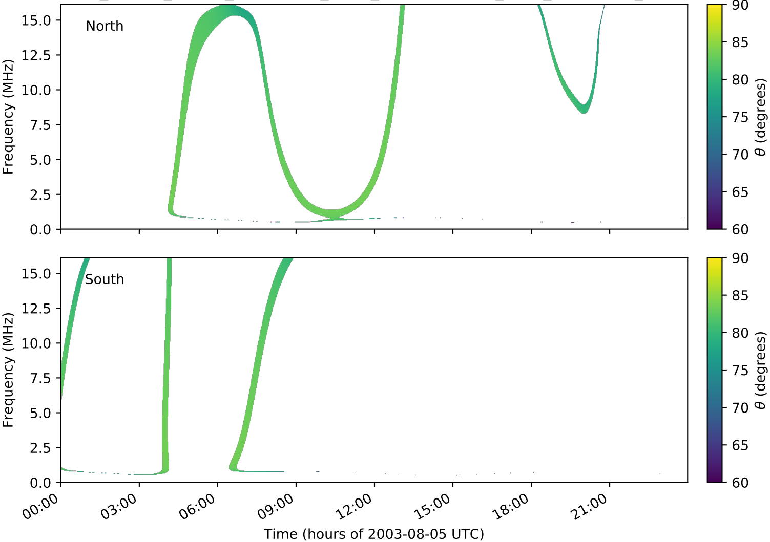
expres_cassini_jupiter_ganymede_isaac_lossc-wid1deg_3kev_20030805_v01.cdf
