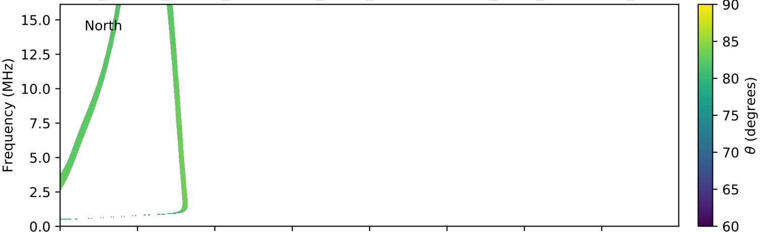
expres_cassini_jupiter_ganymede_isaac_lossc-wid1deg_3kev_20030801_v01.cdf
