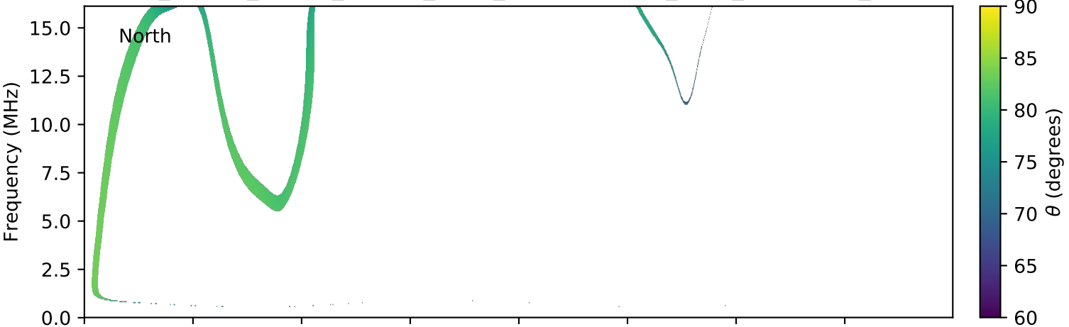
expres_cassini_jupiter_europa_isaac_lossc-wid1deg_3kev_20030830_v01.cdf
