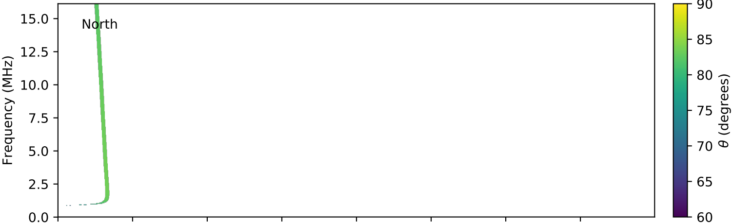
expres_cassini_jupiter_europa_isaac_lossc-wid1deg_3kev_20030828_v01.cdf
