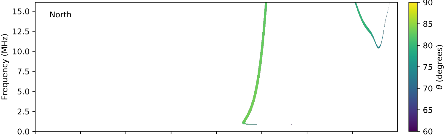
expres_cassini_jupiter_europa_isaac_lossc-wid1deg_3kev_20030826_v01.cdf
