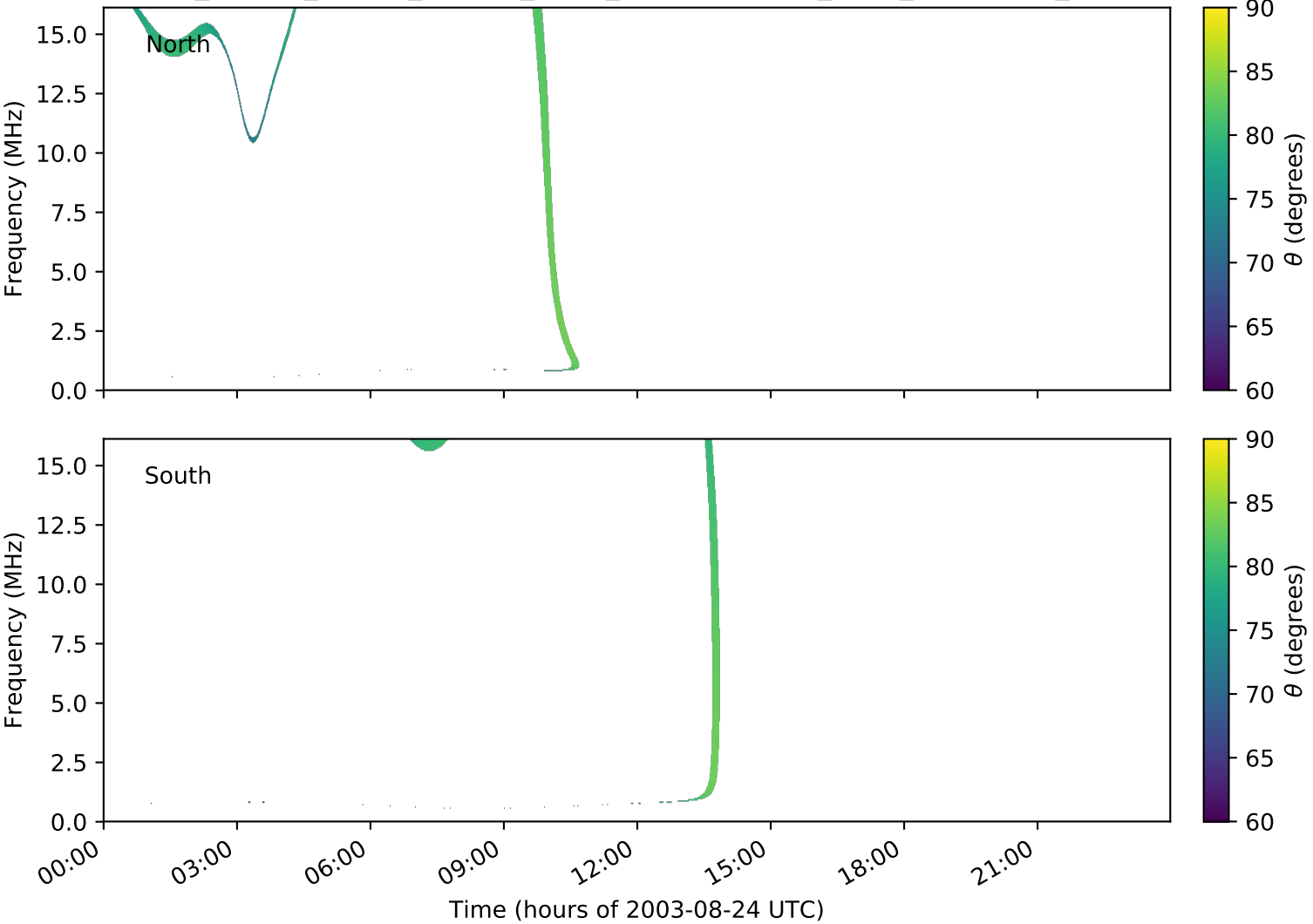
expres_cassini_jupiter_europa_isaac_lossc-wid1deg_3kev_20030824_v01.cdf
