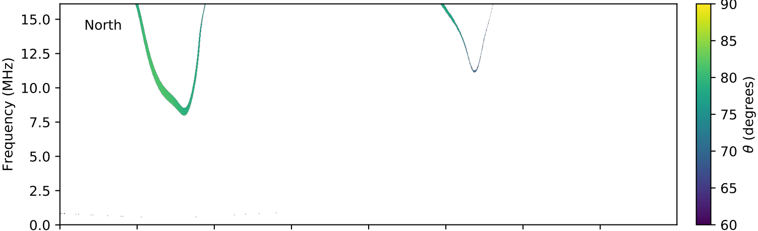
expres_cassini_jupiter_europa_isaac_lossc-wid1deg_3kev_20030823_v01.cdf
