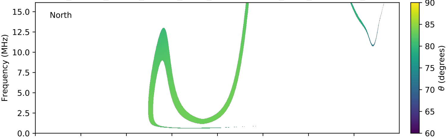
expres_cassini_jupiter_europa_isaac_lossc-wid1deg_3kev_20030819_v01.cdf
