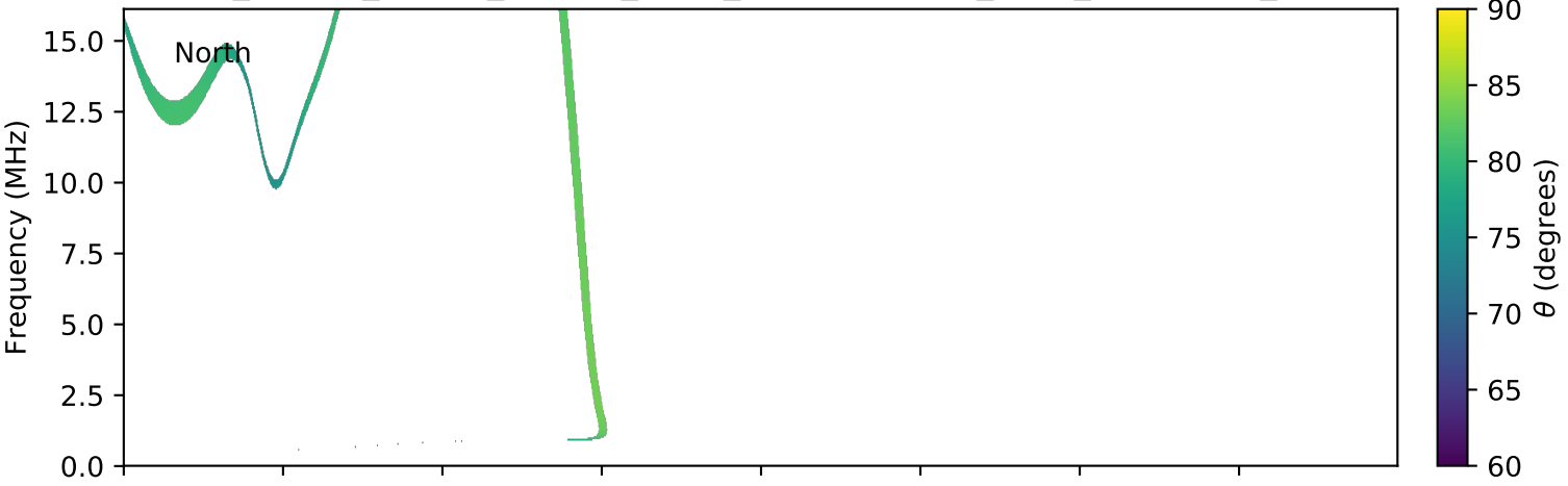
expres_cassini_jupiter_europa_isaac_lossc-wid1deg_3kev_20030817_v01.cdf
