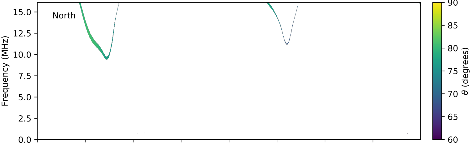
expres_cassini_jupiter_europa_isaac_lossc-wid1deg_3kev_20030816_v01.cdf
