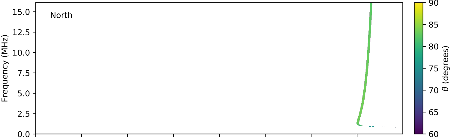
expres_cassini_jupiter_europa_isaac_lossc-wid1deg_3kev_20030815_v01.cdf
