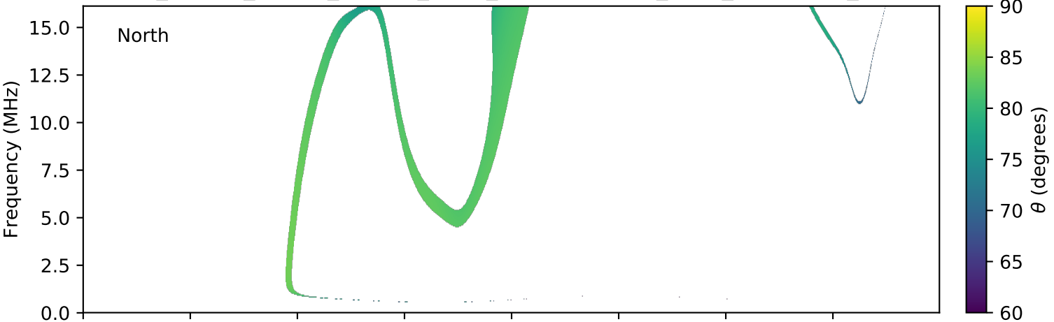
expres_cassini_jupiter_europa_isaac_lossc-wid1deg_3kev_20030812_v01.cdf
