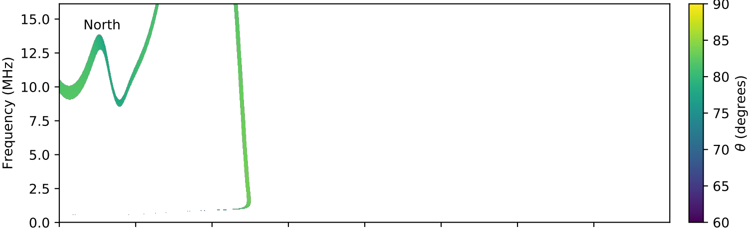
expres_cassini_jupiter_europa_isaac_lossc-wid1deg_3kev_20030810_v01.cdf
