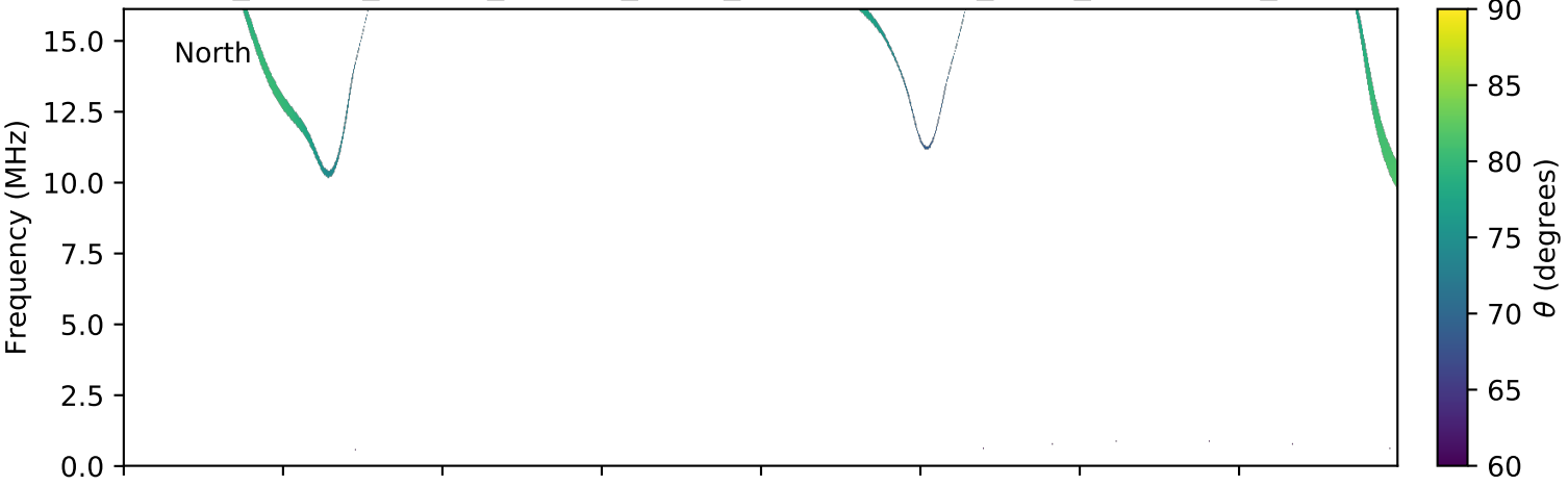
expres_cassini_jupiter_europa_isaac_lossc-wid1deg_3kev_20030809_v01.cdf
