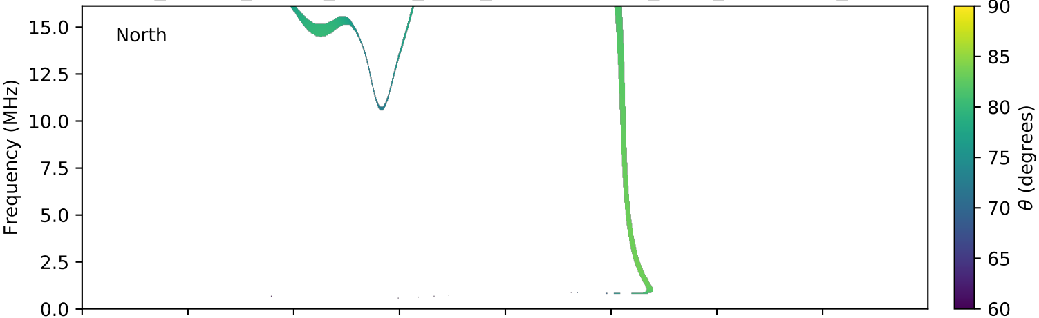
expres_cassini_jupiter_europa_isaac_lossc-wid1deg_3kev_20030806_v01.cdf
