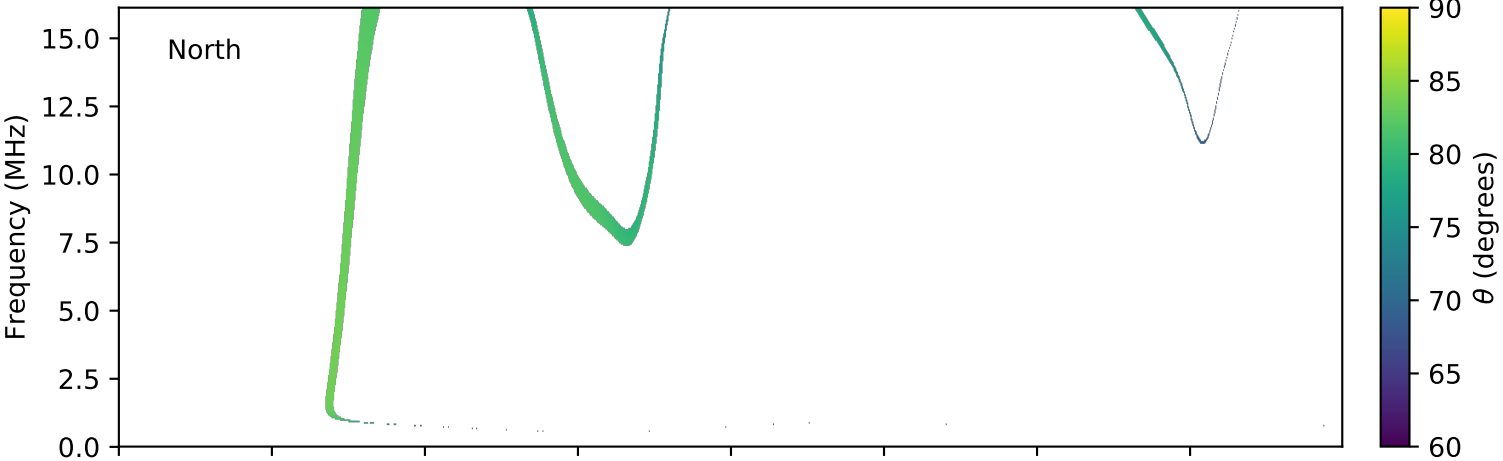
expres_cassini_jupiter_europa_isaac_lossc-wid1deg_3kev_20030805_v01.cdf
