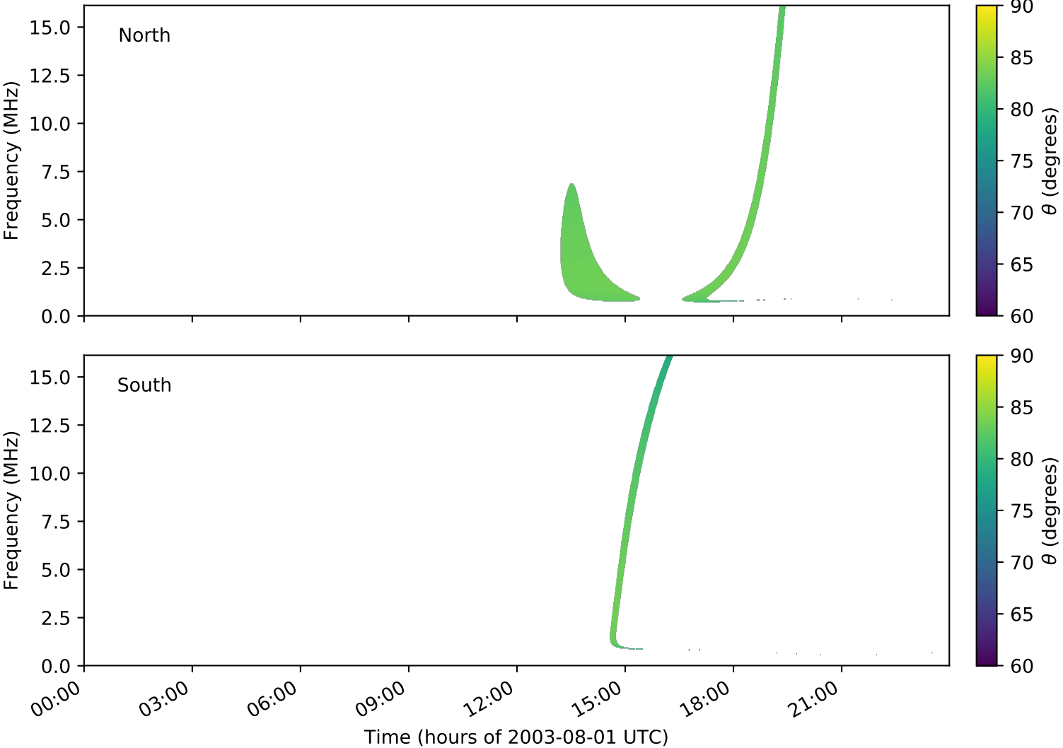
expres_cassini_jupiter_europa_isaac_lossc-wid1deg_3kev_20030801_v01.cdf
