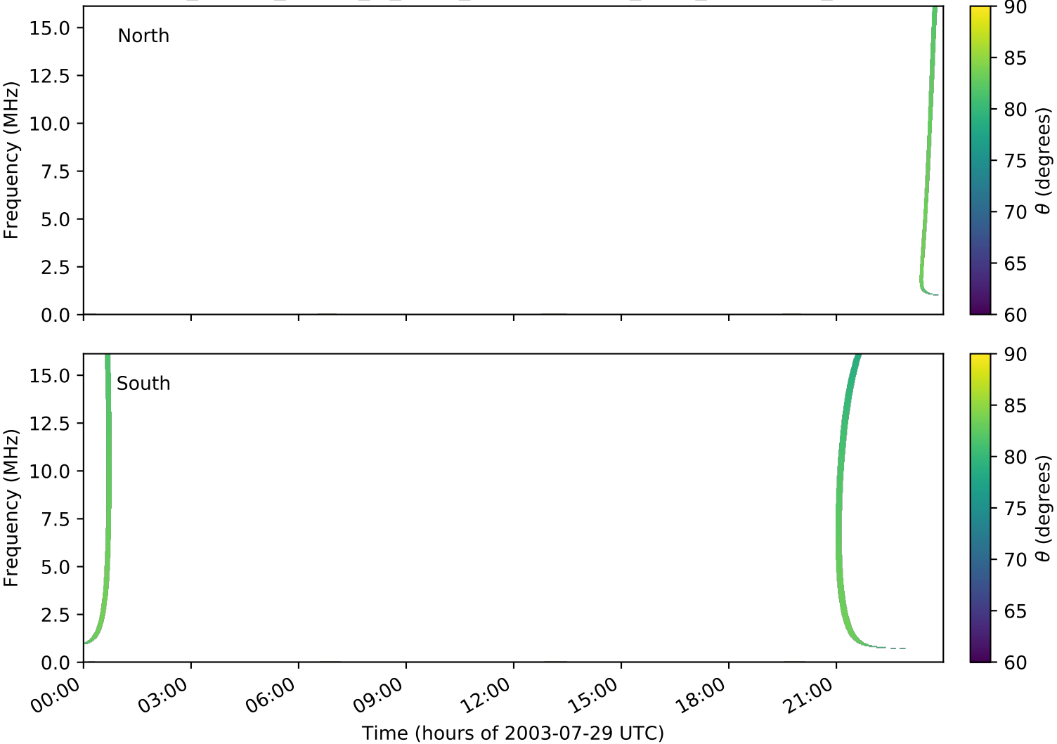
expres_cassini_jupiter_io_isaac_lossc-wid1deg_3kev_20030729_v01.cdf
