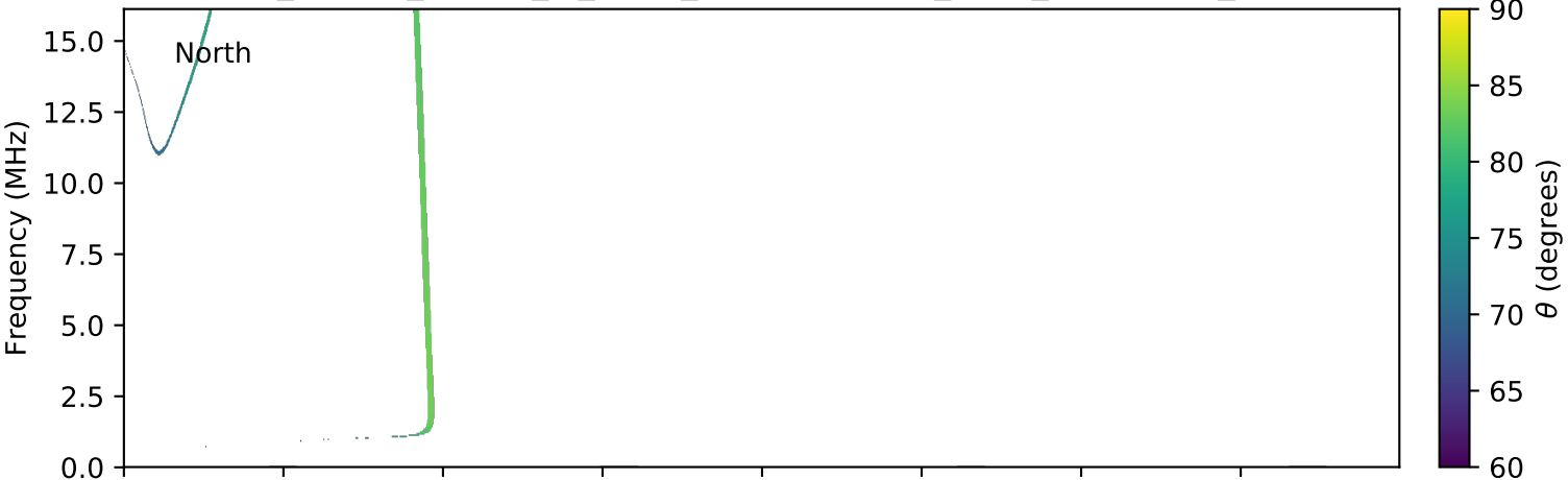
expres_cassini_jupiter_io_isaac_lossc-wid1deg_3kev_20030727_v01.cdf
