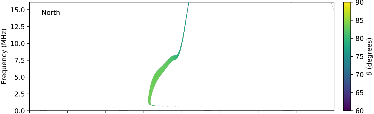
expres_cassini_jupiter_io_isaac_lossc-wid1deg_3kev_20030726_v01.cdf
