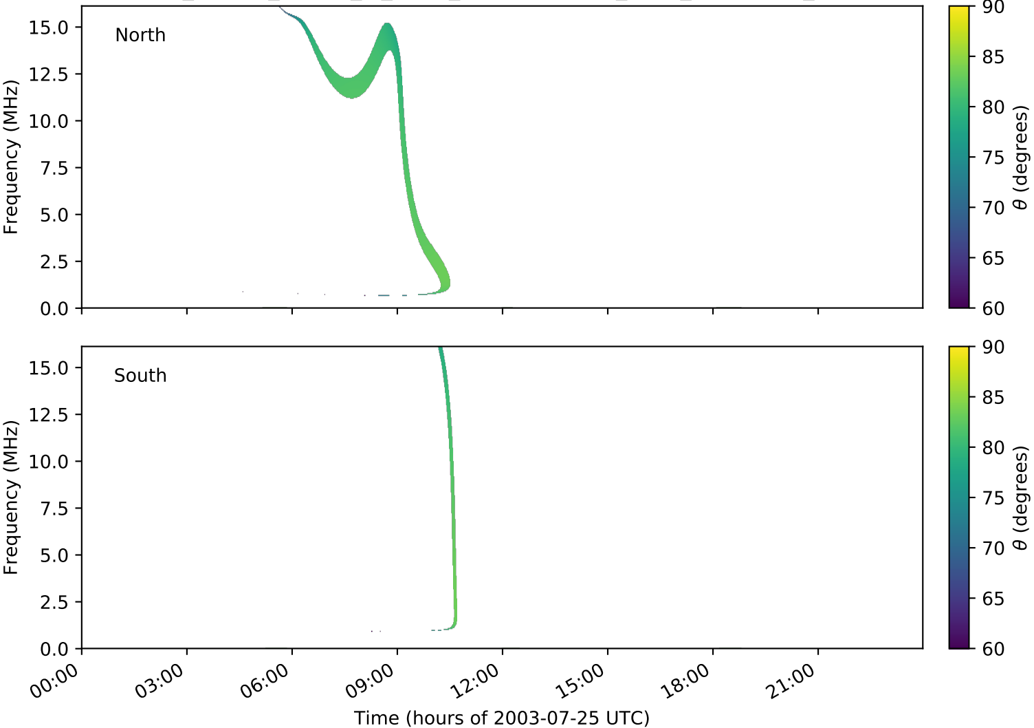
expres_cassini_jupiter_io_isaac_lossc-wid1deg_3kev_20030725_v01.cdf
