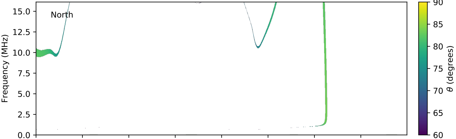
expres_cassini_jupiter_io_isaac_lossc-wid1deg_3kev_20030707_v01.cdf
