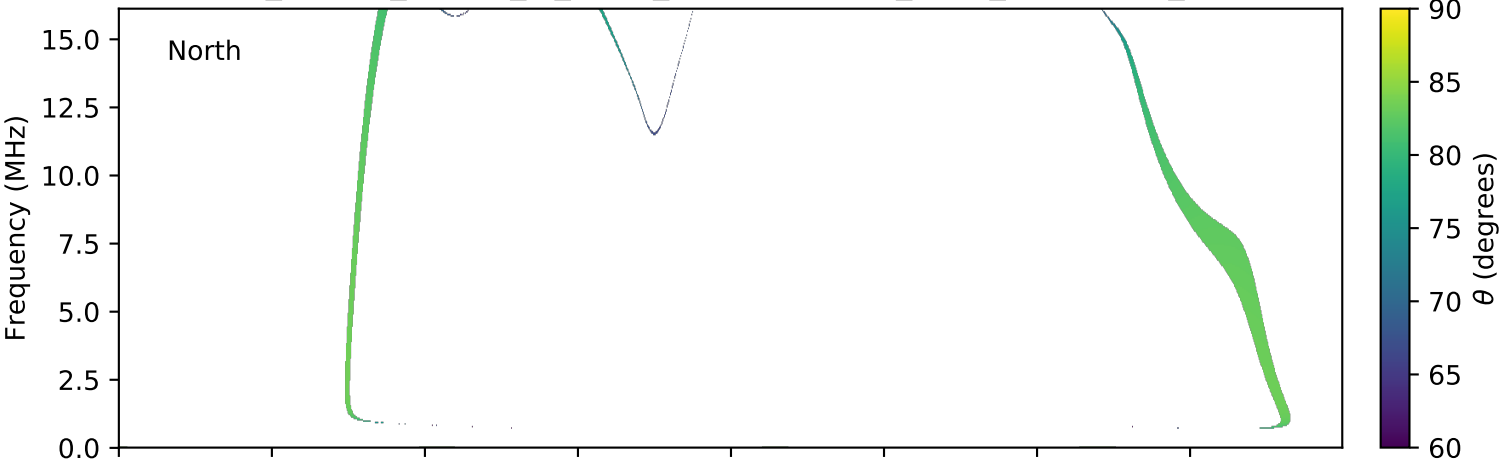
expres_cassini_jupiter_io_isaac_lossc-wid1deg_3kev_20030705_v01.cdf
