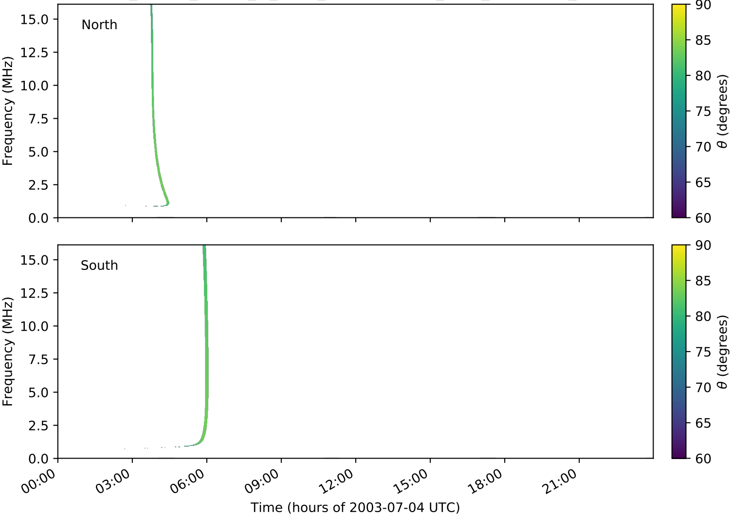
expres_cassini_jupiter_io_isaac_lossc-wid1deg_3kev_20030704_v01.cdf
