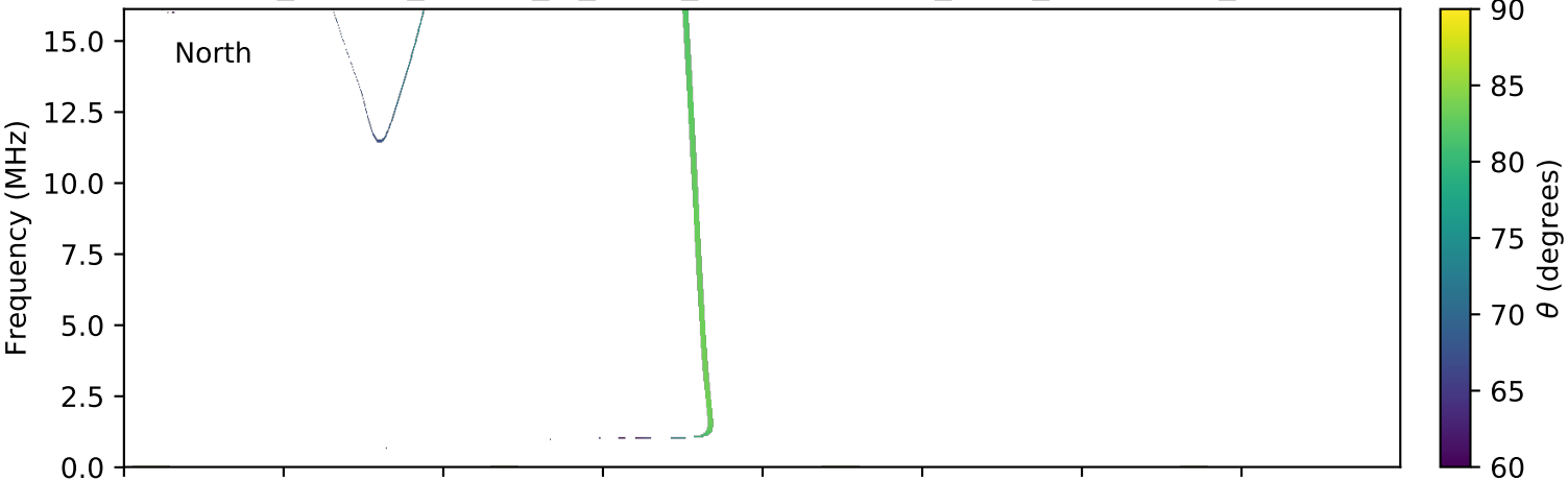
expres_cassini_jupiter_io_isaac_lossc-wid1deg_3kev_20030702_v01.cdf
