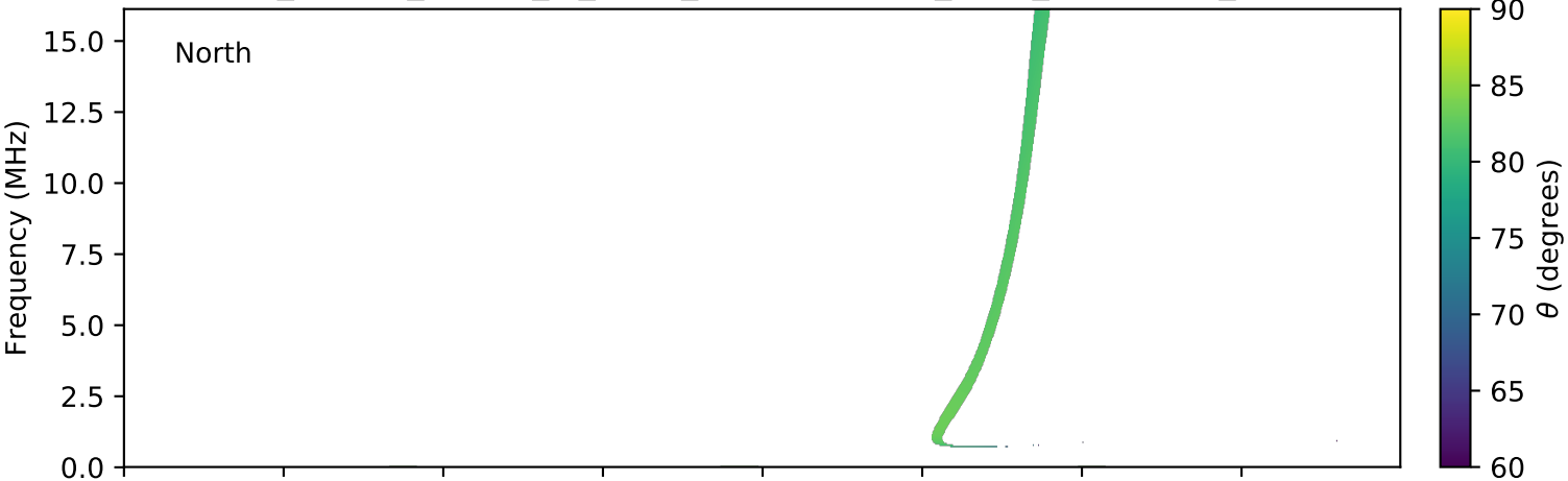
expres_cassini_jupiter_io_isaac_lossc-wid1deg_3kev_20030701_v01.cdf
