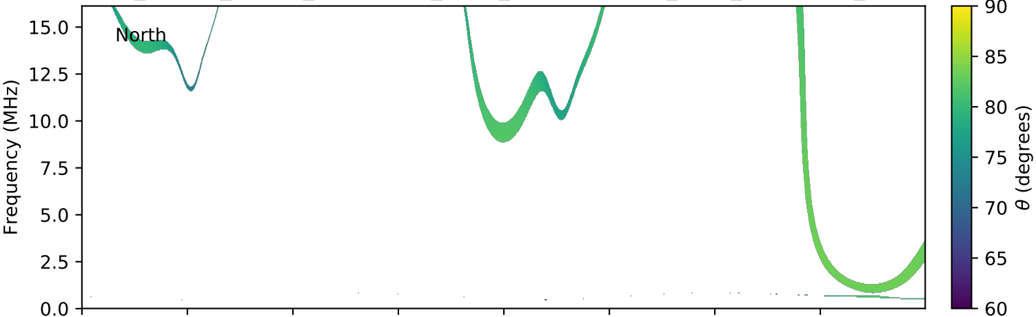
expres_cassini_jupiter_ganymede_isaac_lossc-wid1deg_3kev_20030731_v01.cdf
