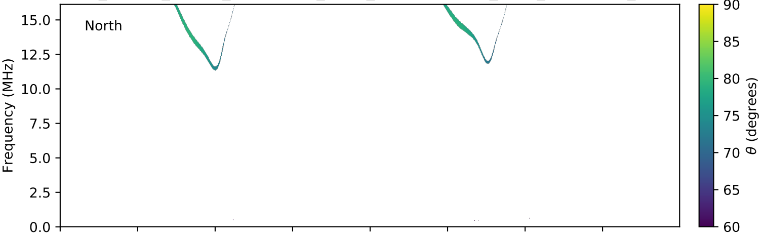
expres_cassini_jupiter_ganymede_isaac_lossc-wid1deg_3kev_20030730_v01.cdf
