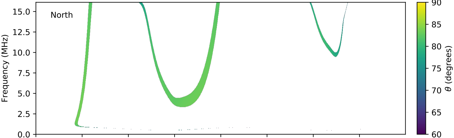
expres_cassini_jupiter_ganymede_isaac_lossc-wid1deg_3kev_20030729_v01.cdf
