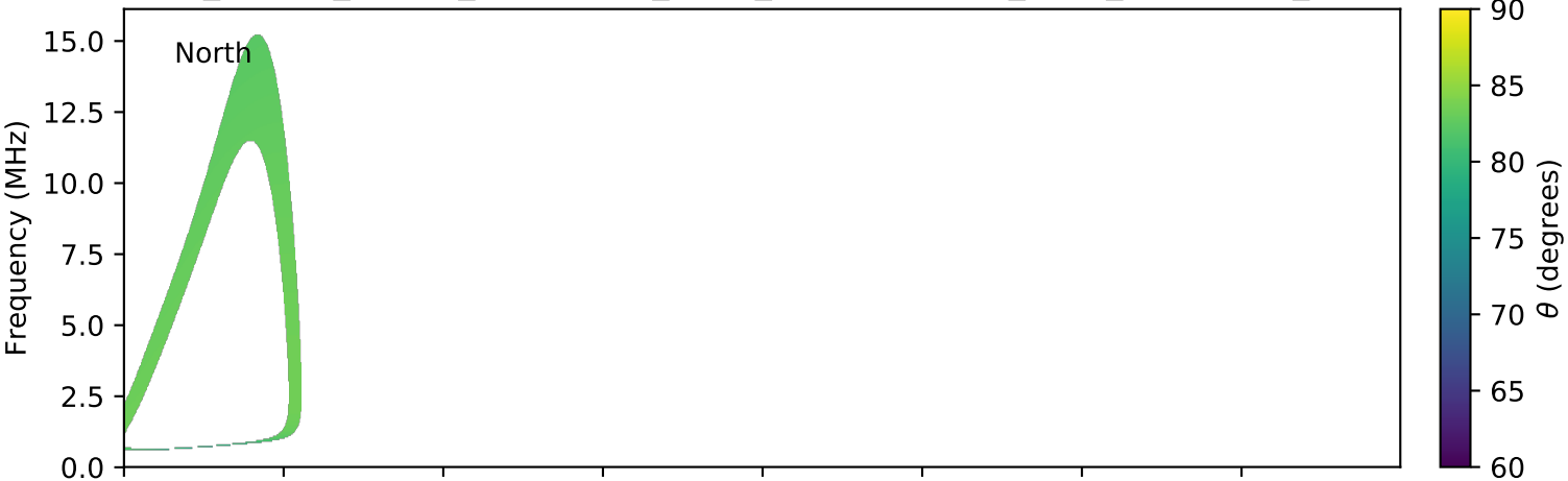
expres_cassini_jupiter_ganymede_isaac_lossc-wid1deg_3kev_20030725_v01.cdf
