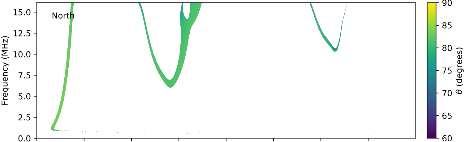
expres_cassini_jupiter_ganymede_isaac_lossc-wid1deg_3kev_20030722_v01.cdf
