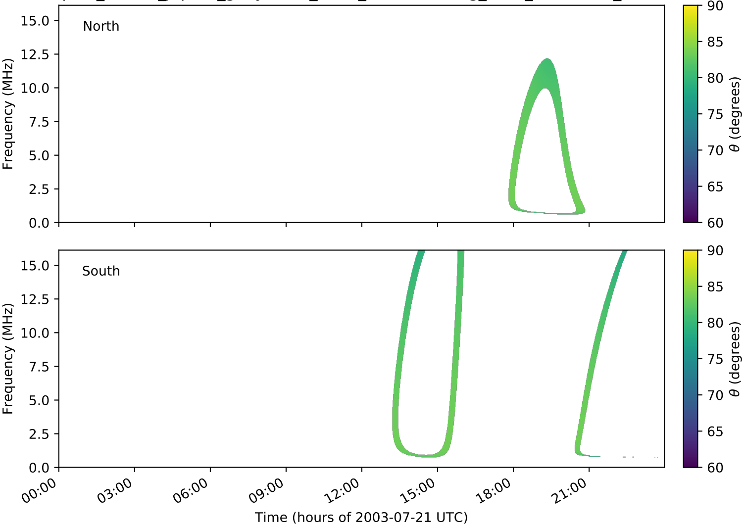
expres_cassini_jupiter_ganymede_isaac_lossc-wid1deg_3kev_20030721_v01.cdf
