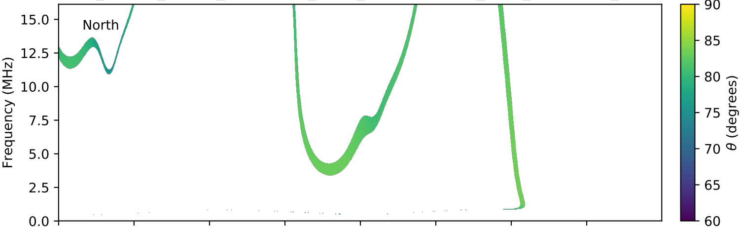
expres_cassini_jupiter_ganymede_isaac_lossc-wid1deg_3kev_20030717_v01.cdf
