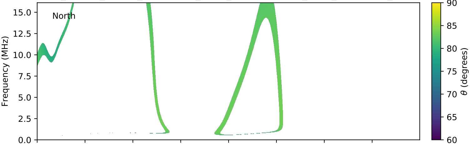
expres_cassini_jupiter_ganymede_isaac_lossc-wid1deg_3kev_20030703_v01.cdf
