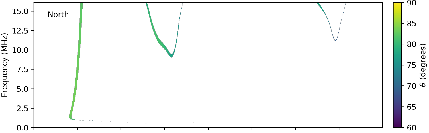
expres_cassini_jupiter_europa_isaac_lossc-wid1deg_3kev_20030729_v01.cdf
