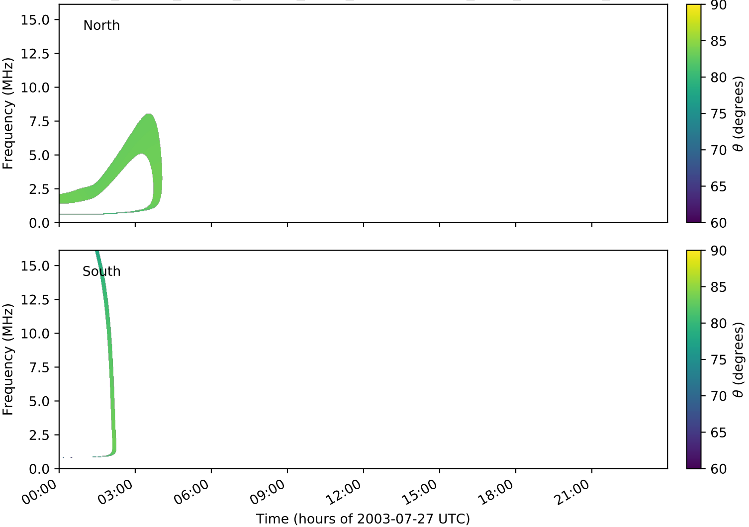
expres_cassini_jupiter_europa_isaac_lossc-wid1deg_3kev_20030727_v01.cdf
