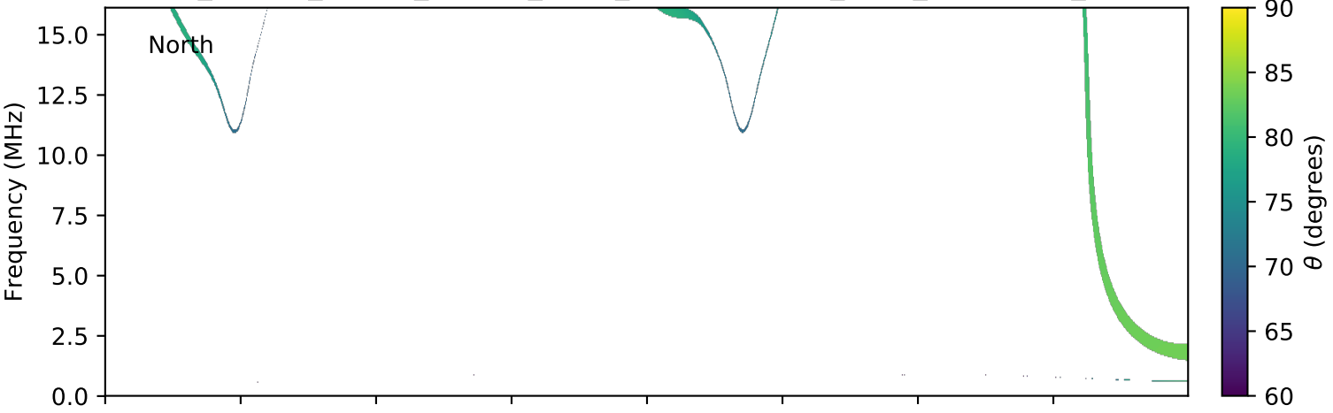
expres_cassini_jupiter_europa_isaac_lossc-wid1deg_3kev_20030726_v01.cdf
