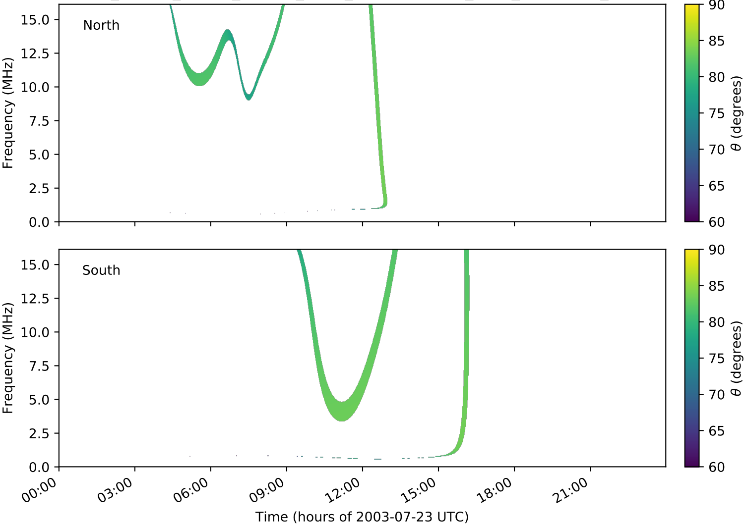
expres_cassini_jupiter_europa_isaac_lossc-wid1deg_3kev_20030723_v01.cdf
