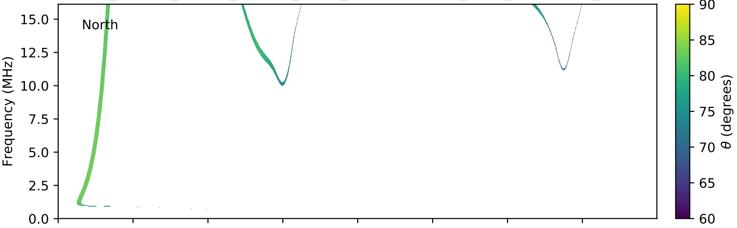
expres_cassini_jupiter_europa_isaac_lossc-wid1deg_3kev_20030722_v01.cdf
