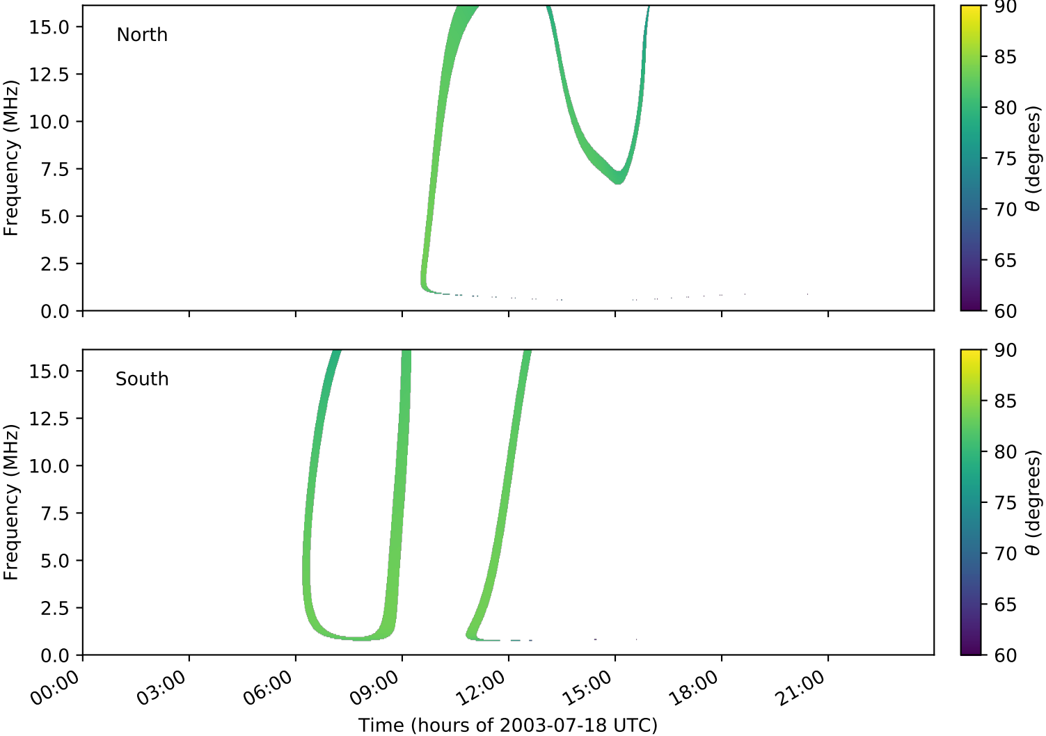
expres_cassini_jupiter_europa_isaac_lossc-wid1deg_3kev_20030718_v01.cdf
