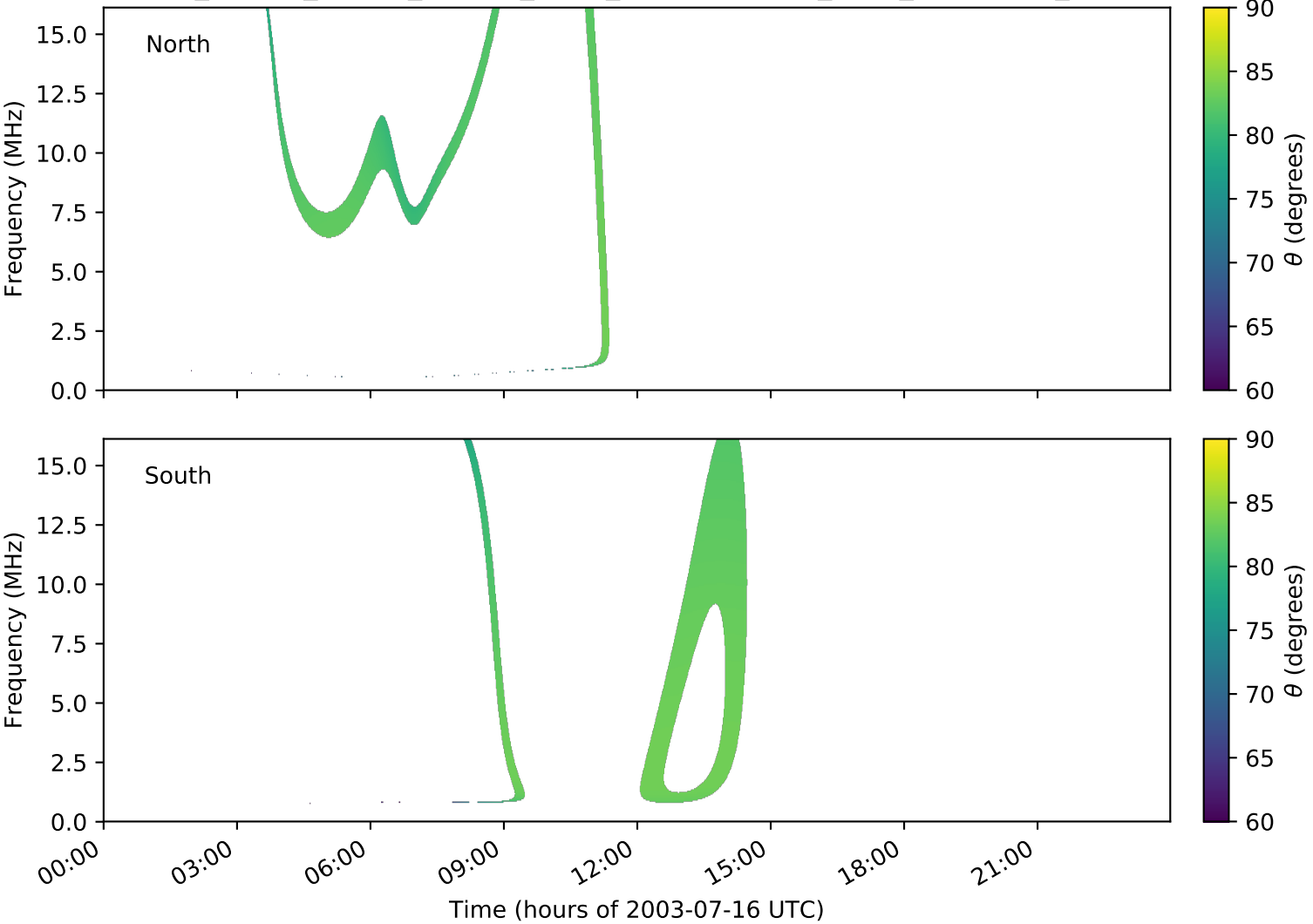
expres_cassini_jupiter_europa_isaac_lossc-wid1deg_3kev_20030716_v01.cdf
