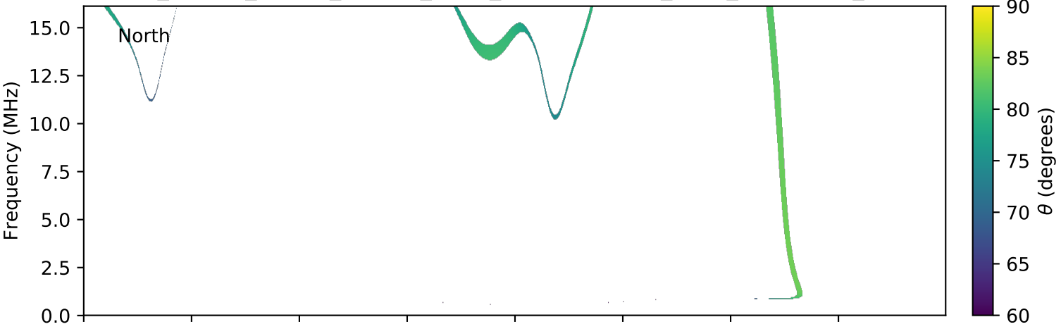
expres_cassini_jupiter_europa_isaac_lossc-wid1deg_3kev_20030712_v01.cdf
