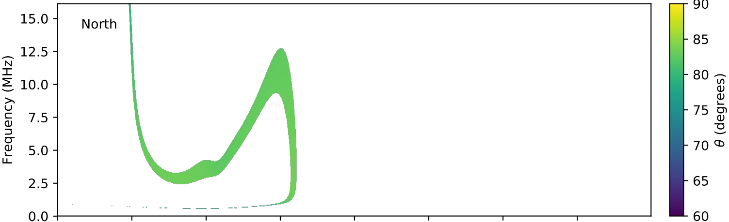
expres_cassini_jupiter_europa_isaac_lossc-wid1deg_3kev_20030709_v01.cdf
