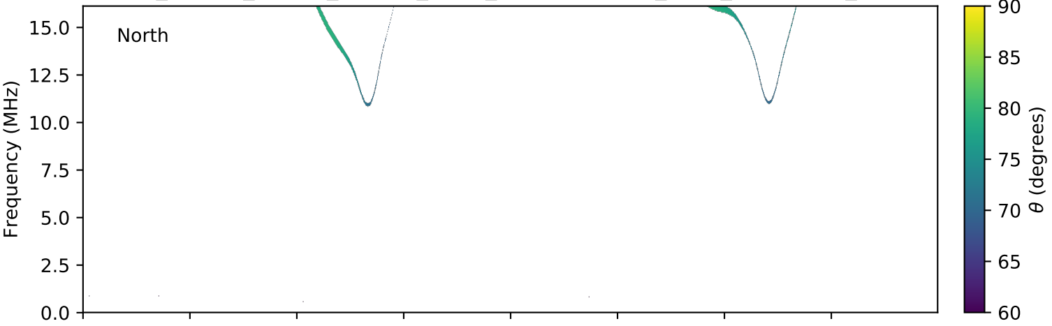
expres_cassini_jupiter_europa_isaac_lossc-wid1deg_3kev_20030708_v01.cdf
